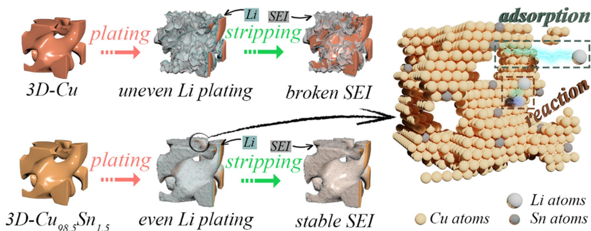
图 3 3D- \text{Cu}_{98.5}\text{Sn}_{1.5} 集流体与纯三维铜集流体表面锂沉积/剥离过程示意图 Figure 3 Schematic Illustration of Lithium Deposition/Stripping on the Surfaces of the 3D \text{Cu}_{98.5}\text{Sn}_{1.5} Current Collector and the Pure 3D Copper Current Collector
