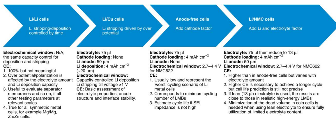
图 4 用于锂金属电池库仑效率测试与结果解析的纽扣电池评测规范 Figure 4 Standardized Coin-Cell Testing Protocol for Coulombic Efficiency Evaluation and Result Interpretation in Lithium-Metal Batteries
