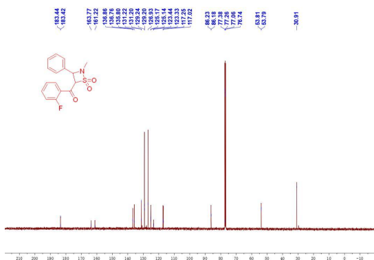
图 15 产物 3ab (2-氟苯基) 的核磁共振碳谱 Figure 15 ^{13}\text{C} NMR spectrum of product 3ab (2-fluorophenyl)
