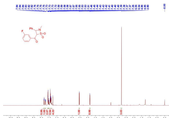
图 17 产物 3ac (3-氟苯基) 的核磁共振氢谱 Figure 17 ^1\text{H} NMR spectrum of product 3ac (3-fluorophenyl)
