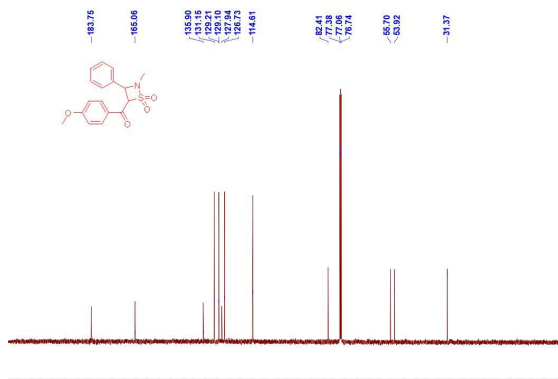
图 30 产物 3ai (4-甲氧基苯基) 的核磁共振碳谱 Figure 30 ^{13}\text{C} NMR spectrum of product 3ai (4-methoxyphenyl)
