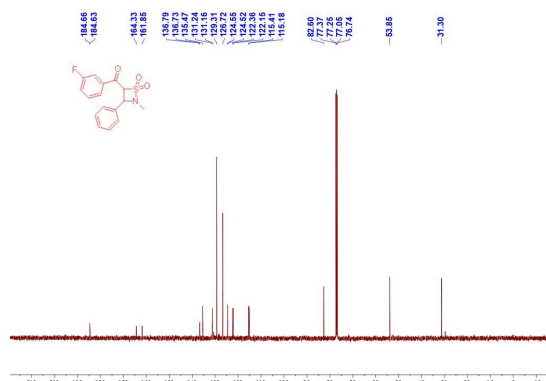
图 18 产物 3ac (3-氟苯基) 的核磁共振碳谱 Figure 18 ^{13}\text{C} NMR spectrum of product 3ac (3-fluorophenyl)
