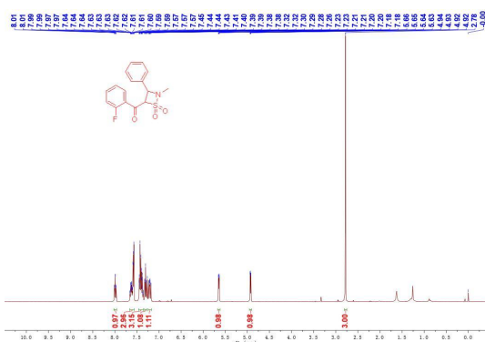
图 14 产物 3ab (2-氟苯基) 的核磁共振氢谱 Figure 14 ^1\text{H} NMR Spectrum of Product 3ab (2-Fluorophenyl)
