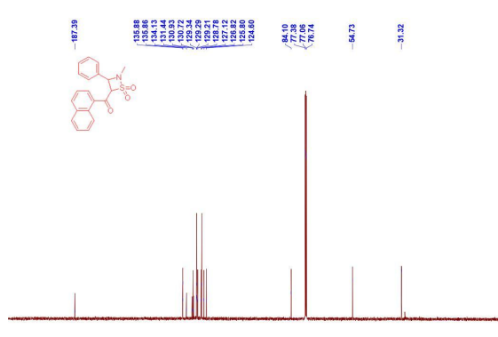
图 34 产物 3ak (萘-1-基) 的核磁共振碳谱 Figure 34 ^{13}\text{C} NMR Spectrum of Product 3ak (Naphthalen-1-yl)
