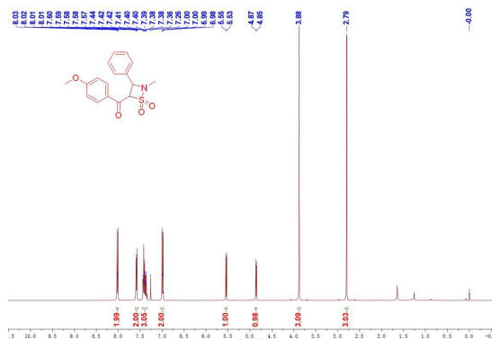
图 29 产物 3ai (4-甲氧基苯基) 的核磁共振氢谱 Figure 29 ^1\text{H} NMR spectrum of product 3ai (4-methoxyphenyl)
