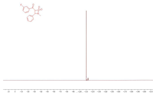
图 19 产物 3ac (3-氟苯基) 的核磁共振氟谱 Figure 19 ^{19}\text{F} NMR spectrum of product 3ac (3-fluorophenyl)
