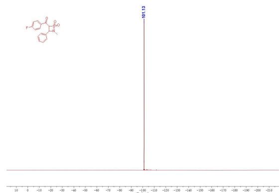
图 22 产物 3ad (4-氟苯基) 的核磁共振氟谱 Figure 22 ^{19}\text{F} NMR spectrum of product 3ad (4-fluorophenyl)
