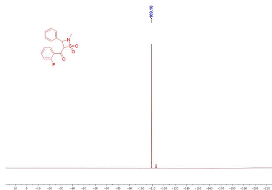
图 16 产物 3ab (2-氟苯基) 的核磁共振氟谱 Figure 16 ^{19}\text{F} NMR spectrum of product 3ab (2-fluorophenyl)
