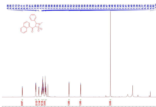
图 33 产物 3ak (萘-1-基) 的核磁共振氢谱 Figure 33 ^1\text{H} NMR spectrum of product 3ak (naphthalen-1-yl)
