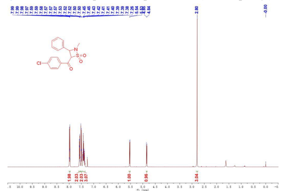
图 23 产物 3ae (4-氯苯基) 的核磁共振氢谱 Figure 23 ^1\text{H} NMR spectrum of product 3ae (4-chlorophenyl)
