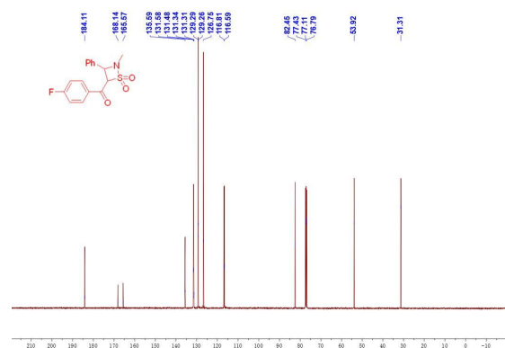
图 21 产物 3ad (4-氟苯基) 的核磁共振碳谱 Figure 21 ^{13}\text{C} NMR spectrum of product 3ad (4-fluorophenyl)
